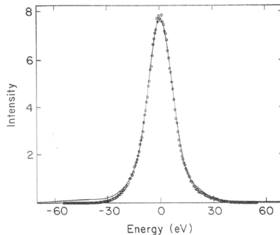
Fig. (16). Resolution function of the toroidal magnetic spectrometer at Zurich University [123]. The solid line with the resolution of 17.0 eV (FWHM) was derived from the measured L_1 conversion-electron line of the 30.898 keV transition in ^{195}\text{Au} ( \Gamma = 6.25 \text{ eV} ). Points were obtained from a Monte Carlo simulation.
