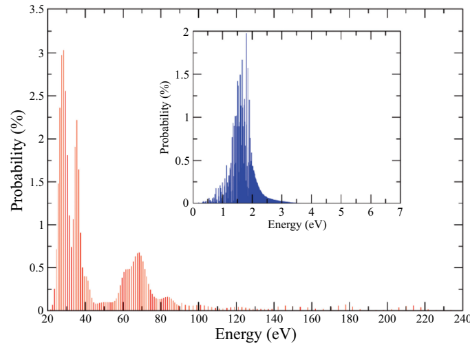
Fig. (6). Probability distribution for excitations of the ( {}^3\text{HeT}^+ ) ion populated the in \beta -decay of gaseous \text{T}_2 [86]. The figure combines results from the calculations of excitation to the electronic bound states [87] and to the electronic continuum [88] of ( {}^3\text{HeT}^+ ). The electronic ground state is populated in 57% of the decays, 29% of the decays end in the excited electronic states and remaining 14% lead to the electronic continuum. The rotational-vibrational excitations of the molecular ion in its ground electronic state are shown in the insert. The mean energy of these excitations is 1.7 eV with the energy spread (FWHM) of about 0.4 eV. The electronic excitations of the ( {}^3\text{HeT}^+ ) ion starting at about 20 eV are shown in the lower part of the figure.
