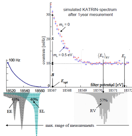
Fig. (17). Upper right: Simulated KATRIN data in the last 5 eV below the endpoint E_0 after 1 year of measurement for neutrino mass 0 eV (upper read crosses) and 0.5 eV (lower blue crosses). Upper left: Schematic increase of the count rate towards the lower energy of \beta -particles. Lower half: EE and RV: Electronic and rotational/vibrational excitation of the daughter molecule ( \text{T}^3\text{He}^+ ) occurring with 43% and 57% probability, resp.; EL: energy loss of 18.5 keV beta's within \text{T}_2 -gas, affecting about 40% of them. The figure is reproduced from [140].
