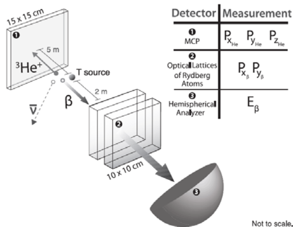
Fig. (24). Diagram illustrating the mechanism of the \beta -decay experiment proposed for the kinematic reconstruction of the neutrino mass from coincident measurement of \beta -particles and {}^3\text{He}^+ ions emitted by ultracold atomic tritium [168].
