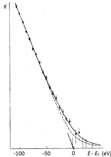
Fig. (13). Kurie plot of the endpoint region of the tritium \beta -spectrum measured with a toroidal magnetic spectrometer by Tretyakov et al [113]. Solid and dashed lines correspond to m_\nu = 0 and 40 eV, respectively.
