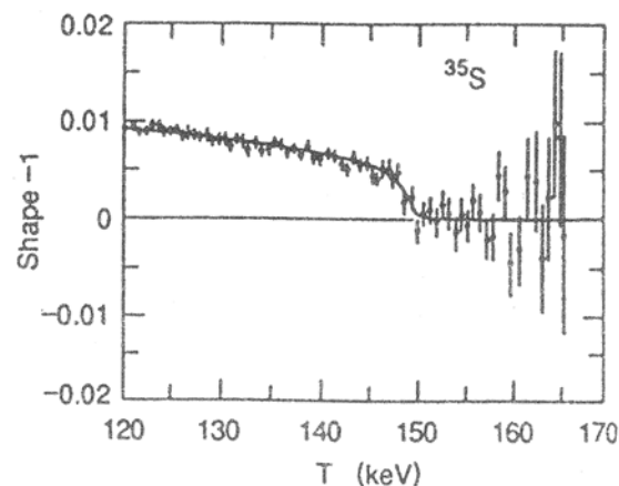
Fig. (27). The shape factor of the \beta -ray spectrum of ^{35}\text{S} measured with a cooled Si(Li) detector [192]. In the energy region of 17 keV below the endpoint of Q_\beta = 167 \text{ keV} , the observed spectrum deviates by 8 standard deviations from the expected single component \beta -spectrum. Solid line includes the 17 keV neutrino mass component with an admixture of 0.0084 \pm 0.0006_{\text{stat}} \pm 0.0005_{\text{sys}} .
