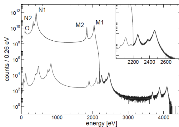
Fig. (19). A Monte Carlo simulation of the calorimetric spectrum of the ^{163}\text{Ho} electron capture decay [151]. Calculations were based on the following assumptions: a decay energy Q_{\text{EC}} = 2200 eV, a neutrino mass m_\nu = 0 , a total number of decay events N_{\text{ev}} = 10^{14} , a microcalorimeter energy resolution \Delta E_{\text{FWHM}} = 2 eV and a pile-up fraction f_{\text{pp}} = 10^{-6} . The bottom curve is a fit of the pile-up spectrum. The insert shows the uppermost part of the spectrum depending on the neutrino mass in a similar way as in the case of the \beta -ray spectra. Note the complexity of the pile-up spectrum at the end of the ^{163}\text{Ho} decay spectrum.
