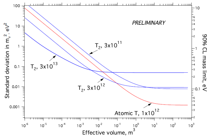
Fig. (21). The neutrino mass sensitivity expected in the Project 8 measurement using cyclotron radiation of single electrons emitted in tritium \beta -decay [161]. The dependence on the effective volume of gaseous sources of molecular or atomic tritium is shown for indicated number densities per \text{cm}^3 . A source temperature will be 30 K for molecular T_2 and 1 K for atomic tritium. Further assumptions were a magnetic field uniformity of 0.1 ppm rms, a background of 10^{-6} \text{ s}^{-1} \text{ eV}^{-1} and a live time of 3 \cdot 10^7 \text{ s} . The m_\nu sensitivity for T_2 is limited to about 100 meV because of the width of the rotational-vibrational states of the (^3\text{HeT})^+ daughter ion and a minimum operating temperature near 30 K.
