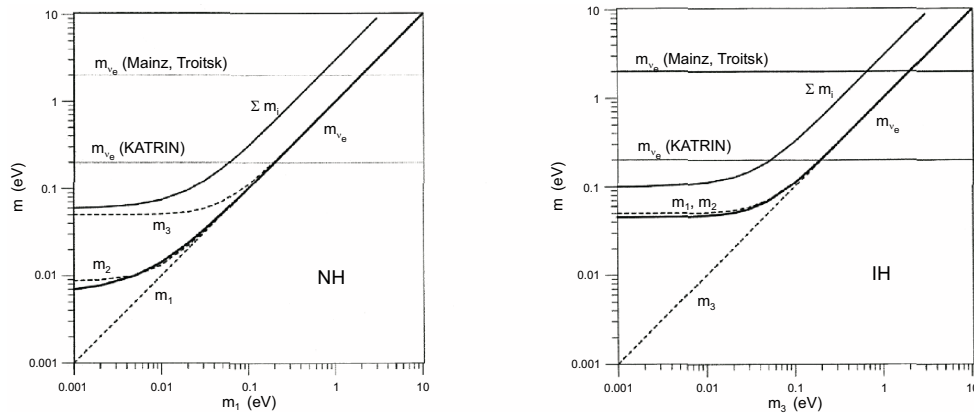
Fig. (1). Neutrino masses m_i as a function of the lightest mass m_1 for the normal hierarchy NH (left panel) and m_3 for the inverted hierarchy IH (right panel). We have calculated the curves for the mean values \Delta m_{21}^2 = 7.53 \cdot 10^{-5} \text{ eV}^2 , |\Delta m_{31}^2| \approx |\Delta m_{32}^2| = 2.44 \cdot 10^{-3} \text{ eV}^2 for NH and 2.52 \cdot 10^{-3} \text{ eV}^2 for IH, and for the admixtures |U_{e1}|^2 = 0.6803 , |U_{e2}|^2 = 0.2354 and |U_{e3}|^2 = 0.0843 derived from [8]. Also shown is the effective neutrino mass m_{\nu_e} , the \beta -spectroscopic quantity defined by Eq. (5), as well as the sum of neutrino masses \sum m_i derived from cosmological measurements. Also depicted is the upper limit of resulting from the latest measurements at Mainz [38] and Troitsk [39] and the expected limit from the upcoming KATRIN experiment [40].
