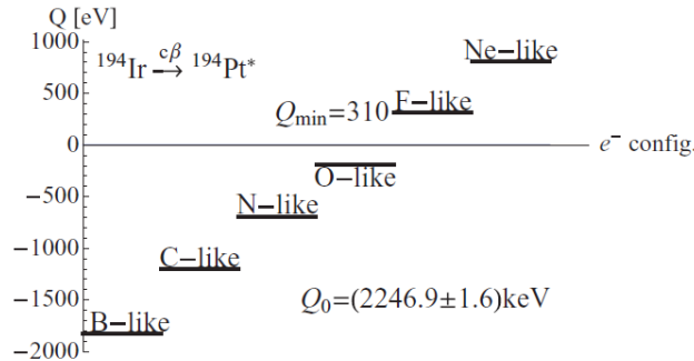
Fig. (23). A change of the iscripts ^{194}_{77}\text{Ir} \rightarrow ^{194}_{78}\text{Pt} \beta^- decay energy by ionization of the parent iridium atom [167]. The figure demonstrates the magnitude of changes but, due to a large uncertainty in the decay energy, it is only illustrative.
