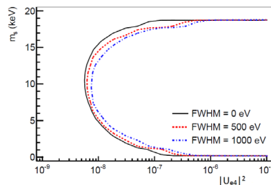
Fig. (33). The 90% exclusion limit for an admixture of keV sterile neutrinos obtained from simulated \beta -spectra [82] that correspond to differential measurements of the KATRIN-like tritium source with a future multi-pixel semiconductor spectrometer of indicated energy resolution.
