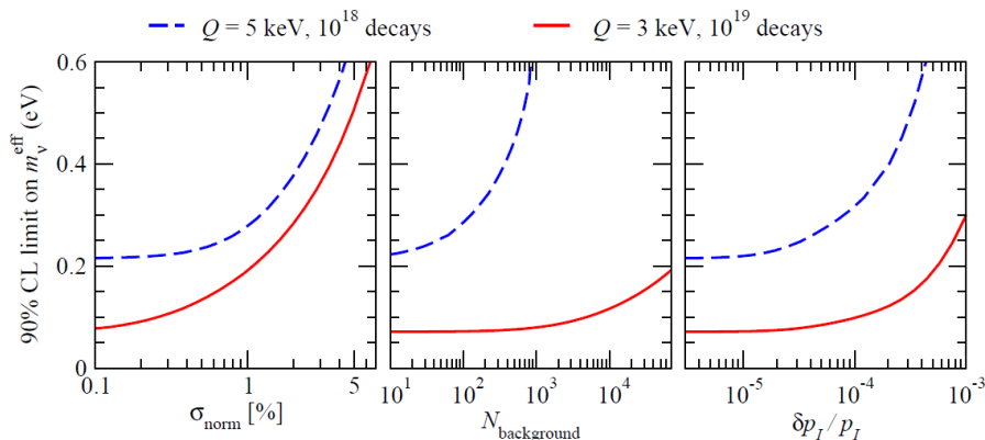
Fig. (22). Sensitivity to the neutrino mass at the 90% CL predicted for the measurement of radioactive ions in a storage ring [166].
