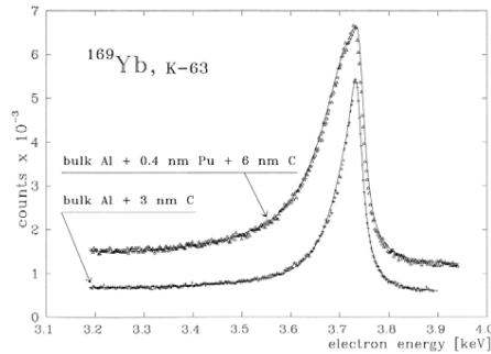
Fig. (30). The K-shell internal-conversion electron line of the 63.1 keV transition in ^{169}\text{Tm} measured with an original and modified ^{169}\text{Yb} source [209]. The original source was prepared by vacuum evaporation onto Al backing and was contaminated by a usual hydrocarbon over layer 21 (described by a 3 nm thick carbon layer in Monte Carlo calculations). In the case of the modified source a supplementary Pu layer of average thickness of 0.4 nm was evaporated where electrons of the kinetic energy of 3.7 keV suffered additional elastic and inelastic scattering. The agreement of measured and calculated (smooth curves) shapes indicates correctness of the electron loss function in plutonium applied in calculations of the ^{241}\text{Pu} \beta -spectrum shape. The natural width of this conversion line is 32.0 eV [212].
