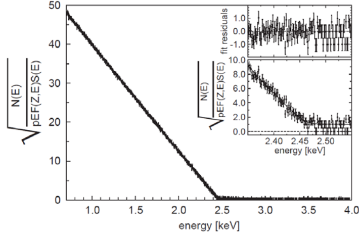
Fig. (18). Kurie plot of the ^{187}\text{Re} (5/2^+) \rightarrow ^{187}\text{Os} (1/2^-) \beta -decay measured with an array of low-temperature microcalorimeters [143]. The least-squares fit of the theoretical spectrum for the first forbidden unique transition yielded a value for \chi^2 per degree of freedom of 0.905. The insert shows the fit of the uppermost part of the \beta -spectrum and the residuals of the fit in units of a standard deviation.
