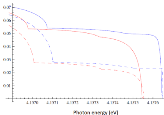
Fig. (25). Relative photon intensity in the threshold regions of the xenon RENP spectrum calculated for Dirac neutrinos assuming two different values of the smallest neutrino mass, 2 and 20 meV [172]. The solid lines correspond to the normal hierarchy ( m_1 < m_2 < m_3 ) and the dashed curves to the inverted hierarchy ( m_3 < m_1 \approx m_2 ) of the neutrino mass states.
