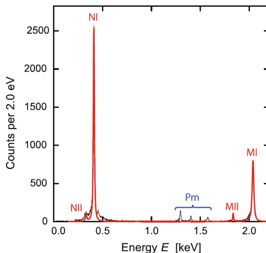
Fig. (20). A spectrum of the ^{163}\text{Ho} electron-capture decay measured by a low temperature calorimeter [156]. The fitted lines are shown in red. Lines labeled Pm correspond to the EC decay of a small amount of ^{144}\text{Pm} admixed in early stage of the ^{163}\text{Ho} measurement.
