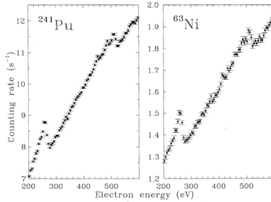
Fig. (31). The KLL-Augur lines of carbon and oxygen superimposed on continuous \beta -spectra of ^{241}\text{Pu} and ^{63}\text{Ni} [214]. The spectra of the vacuum-evaporated sources were recorded with an electrostatic spectrometer [210, 215] by scanning the shown energy regions 10 000 and 18 000 times 22 . The measurement time was 1 s per point in every scan.
