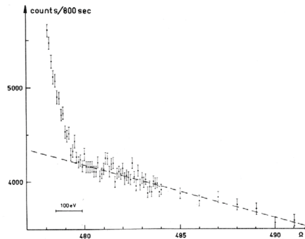
Fig. (10). The endpoint region of the tritium \beta -spectrum measured with the extended source in the Bergkvist experiment [83]. The quantity on the x-coordinate is proportional to the \beta -particle momentum. The spectrum above E_0 was checked for slight curvature by recording the background in the range 480 – 510 \Omega . This test allowed the use of a sloping straight line for background description, as shown.
