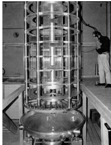
Fig. (15). Toroidal magnetic spectrometer [111] of the Tretyakov type [109] installed at the Zurich University and used in several \beta -decay experiments. Distance between source and detector is 2.65 m. Photo reproduced from [124].
