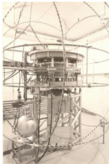
Fig. (11). An iron-free magnetic \beta -ray spectrometer with radial focusing and axial defocusing at the curved exit slit [108]. This focusing principle offers better combination of resolution and transmission than conventional \pi\sqrt{2} spectrometers at the price of a larger detector and focusing angle of (\pi/2)\sqrt{13} = 324.5^\circ . The radius of a central orbit is 30 cm. Note the coils compensating external magnetic fields in three perpendicular directions.
