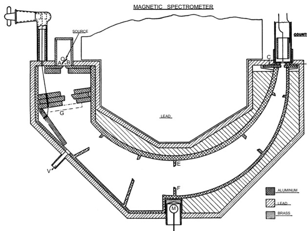
Fig. (8). Magnetic spectrometer [93] with an electron orbit of 40 cm. The iron pole pieces produced the radially inhomogeneous magnetic field that yielded better focus at 180^\circ than a homogenous field. The set of beam-defining slits made of aluminum minimized electron scattering. The instrument was adjusted for the relative momentum resolution 8 of 0.5% and solid angle of about 0.1% of 4\pi . The size of radioactive sources was (0.4 \times 2.5) cm 2 . The energy scale was calibrated with photoelectrons ejected from the K-shell of a lead converter by the 511 keV annihilation radiation.
