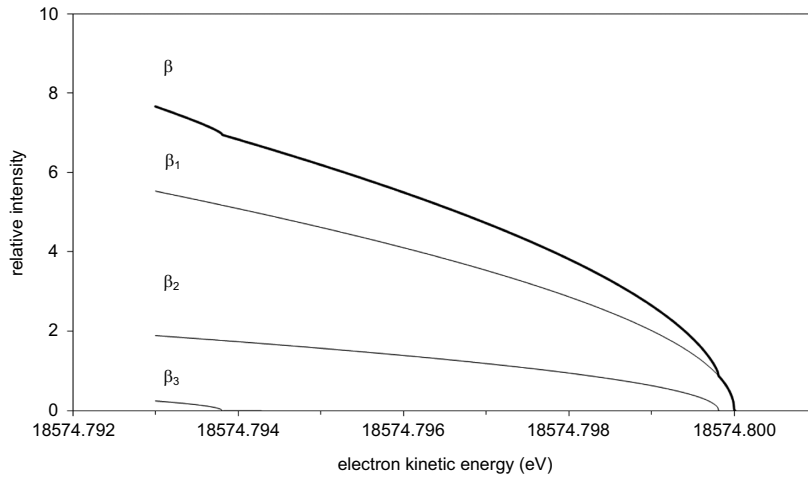
Fig. (7). The uppermost part of the tritium \beta spectrum, wide only 7 meV, was calculated for the normal hierarchy of the neutrino mass states ( m_1 < m_2 < m_3 ) assuming the endpoint energy E_0 = 18.575 keV and m_1 = 200 meV. The same mass square differences \Delta m_{ij}^2 and the admixtures |U_{ei}|^2 as in Fig. (1) were assumed. Under these assumptions m_2 = 200.19 meV, m_3 = 206.19 meV, and the relative intensities of partial spectra \beta_1 , \beta_2 and \beta_3 are |U_{e1}|^2 = 0.6803 , |U_{e2}|^2 = 0.2354 and |U_{e3}|^2 = 0.0843 , respectively [8]. The experimentally observable \beta -spectrum is composed of the three components. Taken with sufficiently high instrumental resolution, the spectrum will exhibit kinks at energies E_0 - m_i ( i = 2, 3 ). In our example, the average electron neutrino mass m_\nu defined by Eq. (5) equals 200.57 meV. We have assumed for simplicity that all the ^3\text{H} \rightarrow ^3\text{He} + e^- + \bar{\nu}_e decays proceed to the ground state of the daughter ion.
