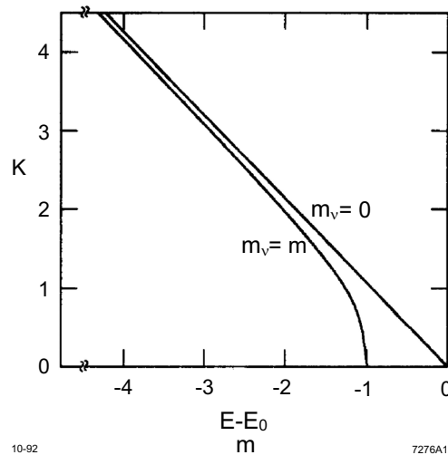
Fig. (5). Kurie plots for an allowed \beta -decay and two values of m_e demonstrating narrowness of the endpoint region sensitive to the neutrino mass [35]. The graphs are obtained from Eq. (9) expressing the parameter E - E in units of m equaled to assumed nonzero value of m_\nu . Explicitly K \cong (E - E_0)/m \times [1 - m^2/(E - E_0)^2]^{1/4} for m_\nu \neq 0 and K \cong (E - E_0)/m for m_\nu = 0 .
