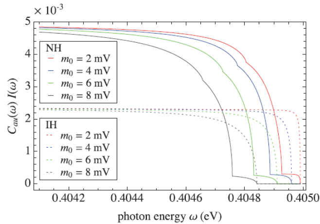
Fig. (26). Endpoint region of the photon RENP spectrum of the iodine molecule calculated for Majorana neutrinos with indicated values of the smallest neutrino mass m_0 [174]. Solid and dashed curves correspond to the normal (NH) and inverted (IH) hierarchy of neutrino mass states. The CP-conserving Majorana with both phases equal to zero was assumed.
