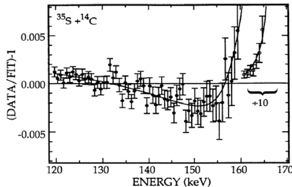
Fig. (29). Residuals from fitting the ^{35}\text{S} \beta -spectrum shape into a measured \beta -spectrum of the composite ( ^{35}\text{S} + ^{14}\text{C} ) source [194]. The solid curve indicates residuals expected from the known admixture of ^{14}\text{C} .
