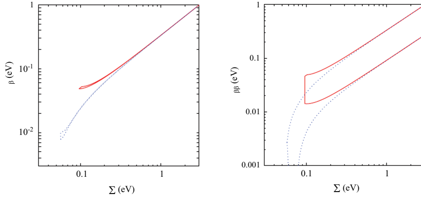
Fig. (3). Regions of the three observables sensitive to the absolute neutrino masses that are allowed by the neutrino oscillation experiments: m_{\beta\beta} \equiv m_{\nu_e} (Eq. 5), m_{\beta\beta} (Eq. 2) and \Sigma m_i for NH (blue dotted) and IH (red solid). Bands correspond to 3\sigma uncertainties of the oscillation data. Figure is reproduced from [81].
