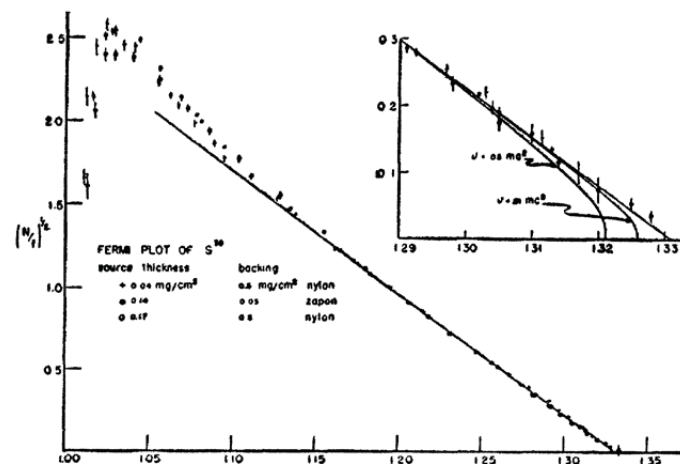
Fig. (9). The Kurie plot of the \beta -spectrum of ^{35}\text{S} measured by Cook et al. [92]. The plots shown correspond to the ^{35}\text{S} sources of estimated thickness of 0.04, 0.14 and 0.17 \text{mg cm}^{-2} that were prepared on 0.5 \text{mg cm}^{-2} Nylon and 0.03 \text{mg cm}^{-2} Zapon backings. For electron energies above 90 keV, the Kurie plots are all straight lines as expected for the ^{35}\text{S}(3/2^+) \rightarrow ^{35}\text{Cl}(3/2^+) \beta -transition. According to the authors the deviations for energies below 60 keV are influenced by source thickness and backing. The enlarged section of the Kurie plot close to the \beta -spectrum endpoint shows the theoretical Fermi curves for an allowed \beta -transition calculated for assumed neutrino masses of 0, 5 and 10 keV.
