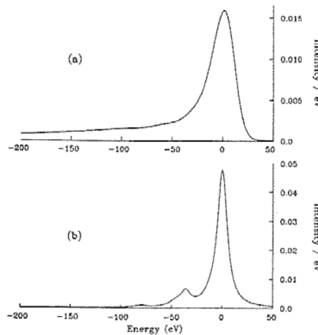
Fig. (14). (a) The overall response function of the experiment [122] obtained from the measured \text{KL}_2\text{L}_3 Auger line by means of Eq. (13). The low-energy tail extends up to -1000 eV. The total intensity is normalized to one. (b) The calculated shake up/off spectrum convoluted with a Lorentzian corresponding to the natural line width \Gamma = 11.43 eV. The peak at the energy loss of 0 eV corresponds to the no-energy-loss component whose probability is 80%.
