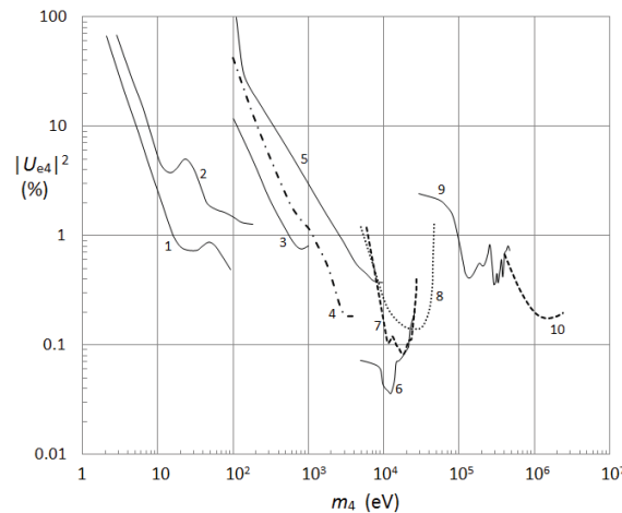
Fig. (32). Best upper limits on the admixture |U_{e4}|^2 of sterile neutrinos derived from measured \beta -ray spectra. All upper limits refer to the 95% CL except those for ^{64}\text{Cu} [186] and ^3\text{H} [219] that were published at the 90% CL. The numbers denote the following radionuclides and their investigators: 1 – ^3\text{H} [218], 2 – ^3\text{H} [219], 3 – ^{187}\text{Re} [206], 4 – ^3\text{H} [203], 5 – ^3\text{H} [114], 6 – ^{63}\text{Ni} [204], 7 – ^{63}\text{Ni} [193], 8 – ^{35}\text{S} [194], 9 – ^{64}\text{Cu} [186], 10 – ^{20}\text{F} [189].
